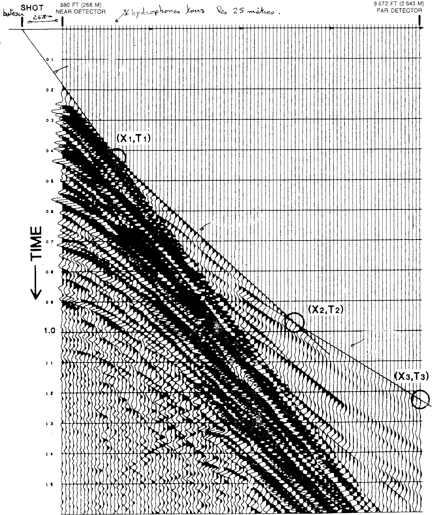
FIG. 2. A shot-ordered file. Straight lines are hand-fitted to first-arrival times, and hand-picked for computer input by their intersections (X_1, T_1) , etc. Streamer length was 2 400 m (7 874 ft).
